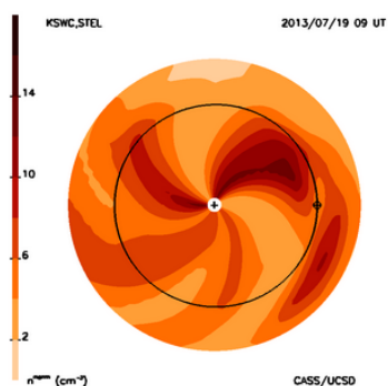
Fig1. Solar Wind Density
