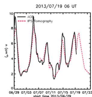
Fig2. Solar wind Density compared with ACE
