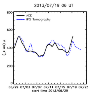
Fig4. Solar wind Velocity compared with ACE
