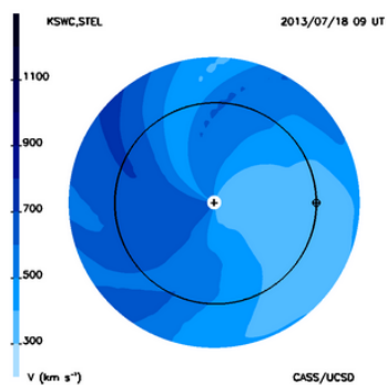
Fig3. Solar wind velocity
